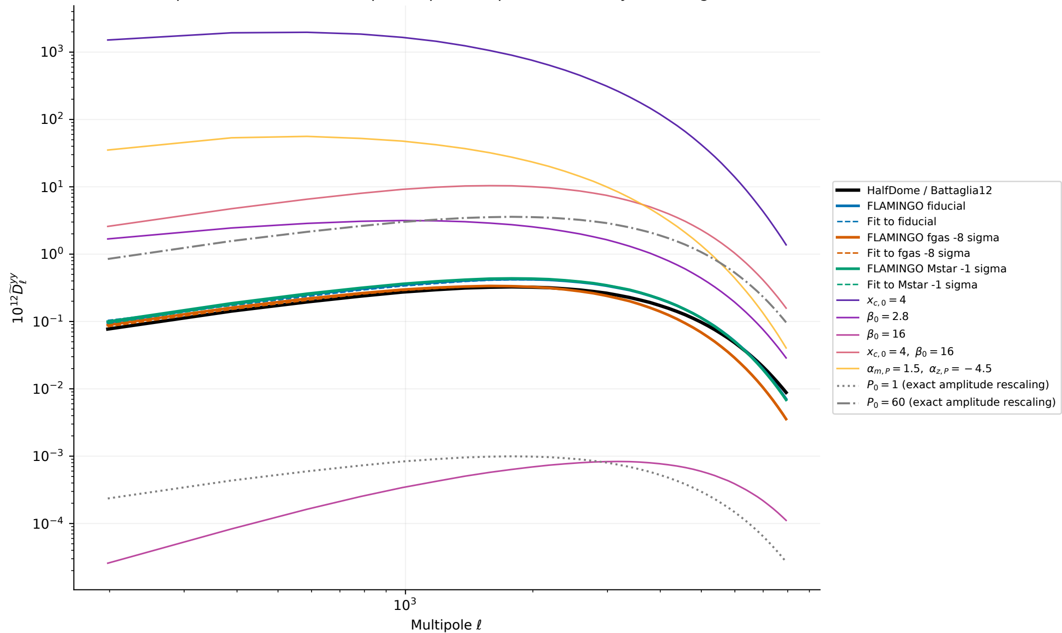
tSZ power across the proposed range Shape extremes use full maps; unspecified parameters stay at Battaglia12
