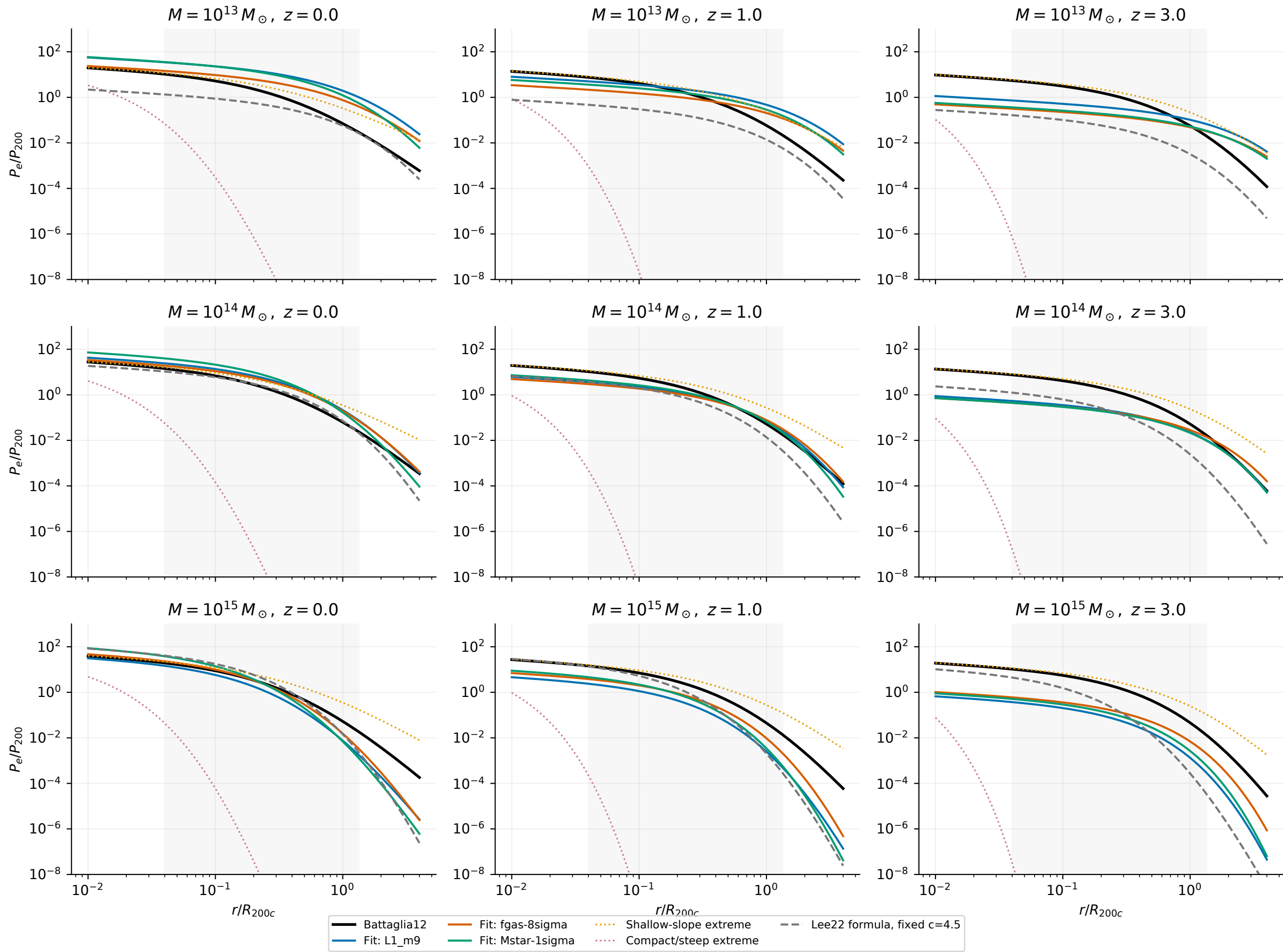
Pressure profiles implied by the spectral fits and extremes Grey band: Lee22 radial fit interval; mass calibration roughly 1.5e13 – 1.5e14 Msun, z \leq 2 Other masses, redshifts and radii are illustrative extrapolations
