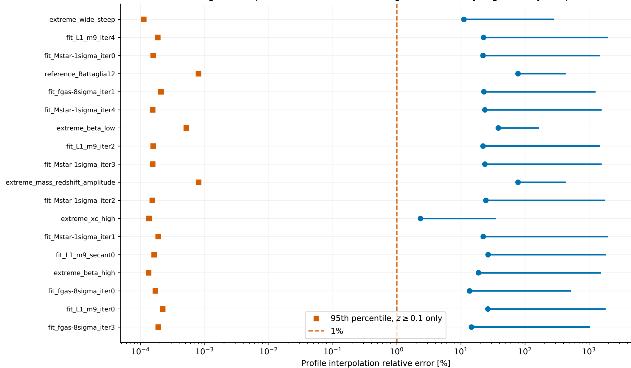
Independent LOS quadrature versus production interpolation Blue: all-grid 95th percentile to maximum; orange: z \geq 0.1 only; significant y samples
