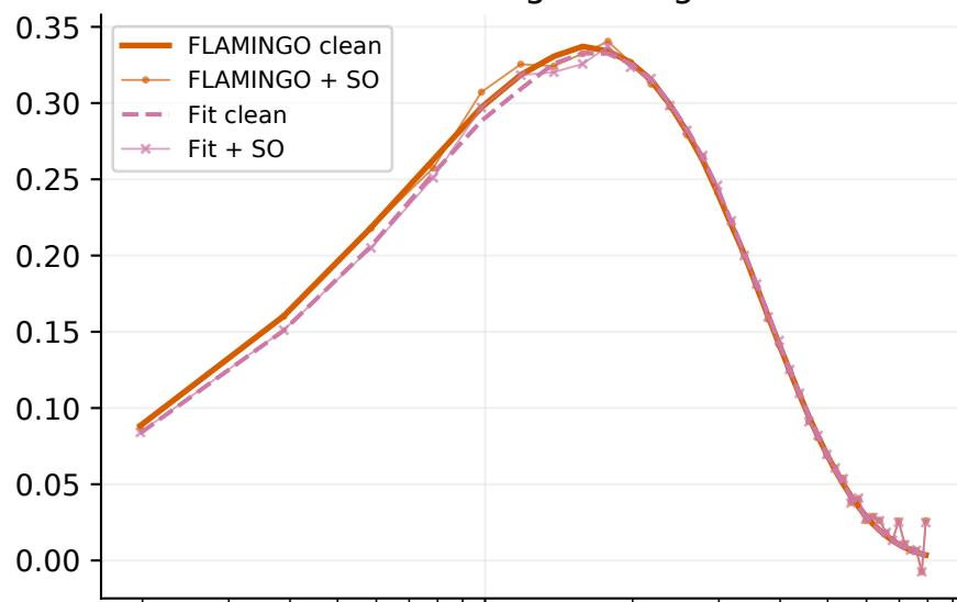
FLAMINGO fgas -8 sigma
