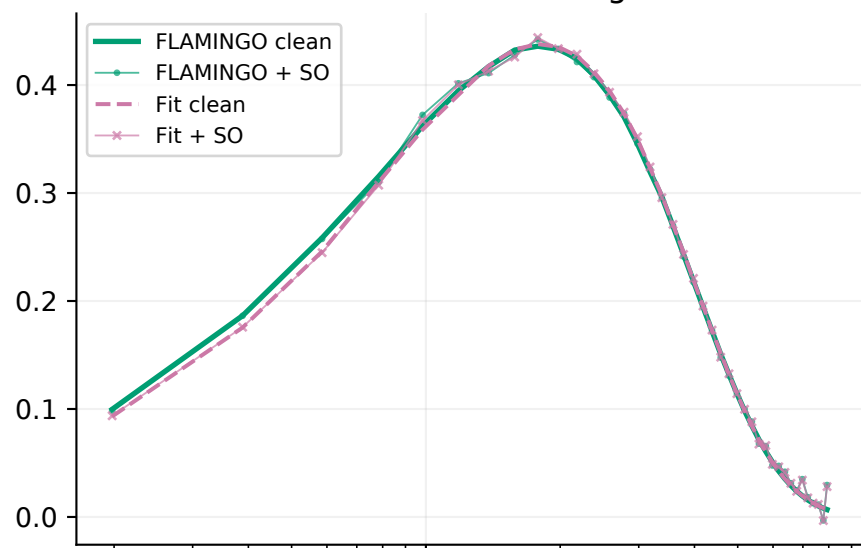
FLAMINGO Mstar -1 sigma
