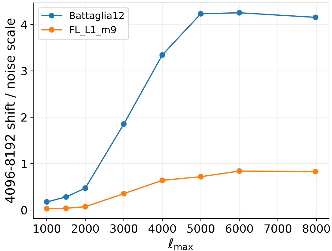
Frozen unbinned MOPED
