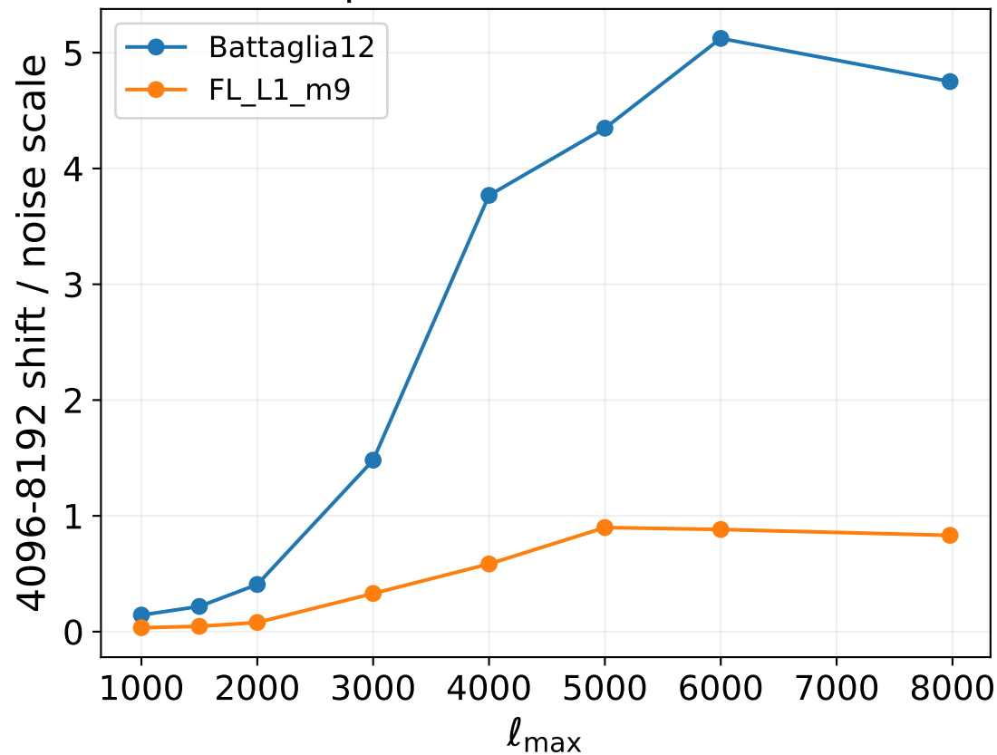
Independent covariance half
