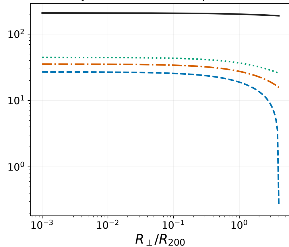
Very shallow outskirts: \beta = 0.644
