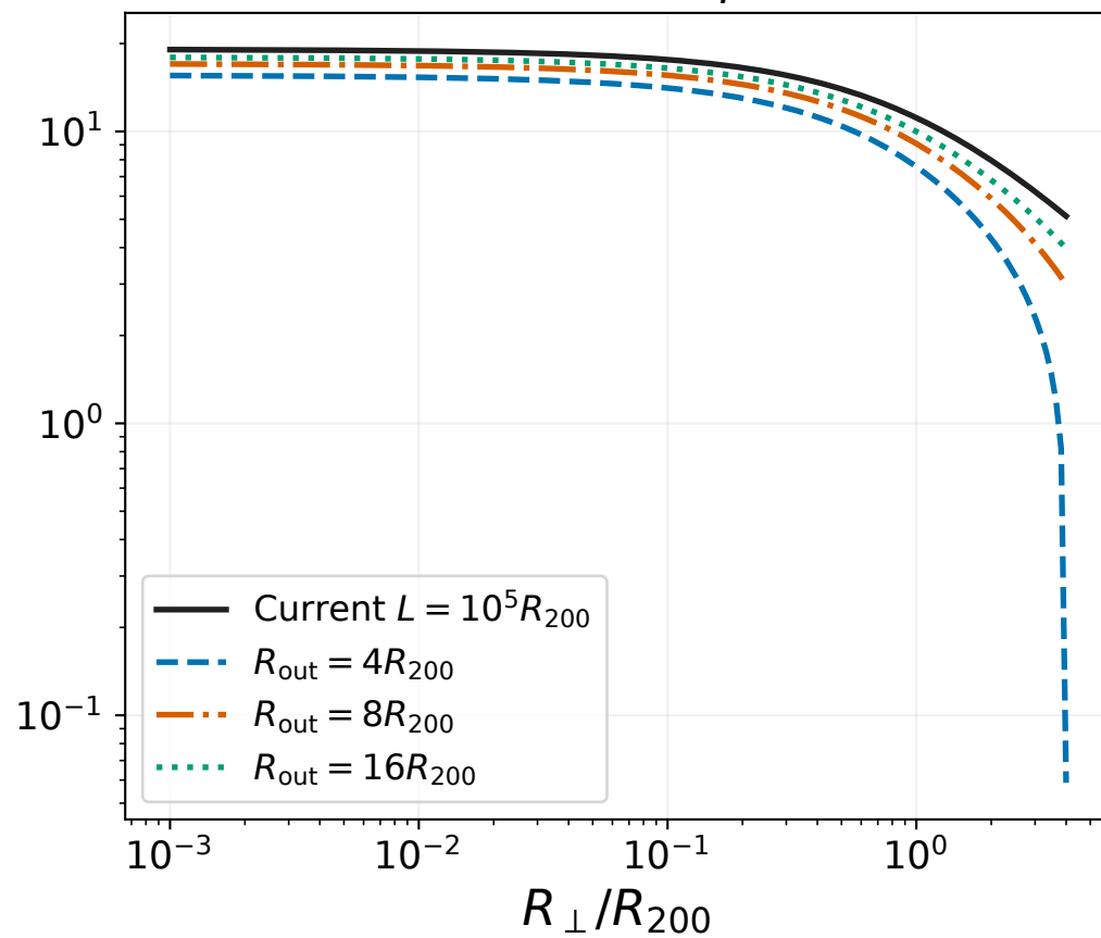
Shallow outskirts: \beta = 1.617
