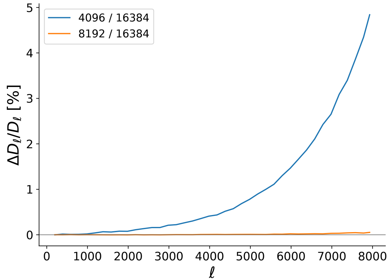
FLAMINGO fiducial fit
