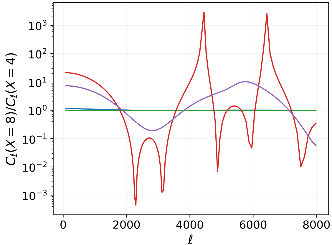
\theta_{200c} = 1 arcmin
