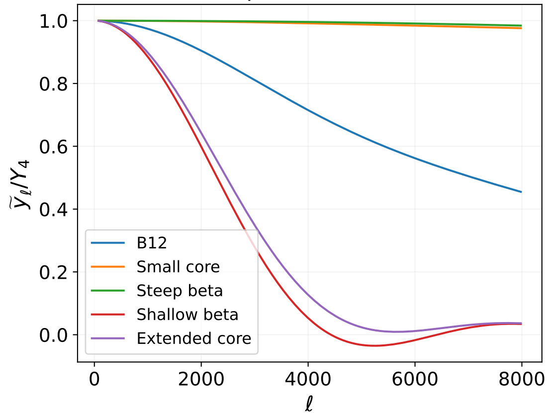
Sphere 4R_{200c}
