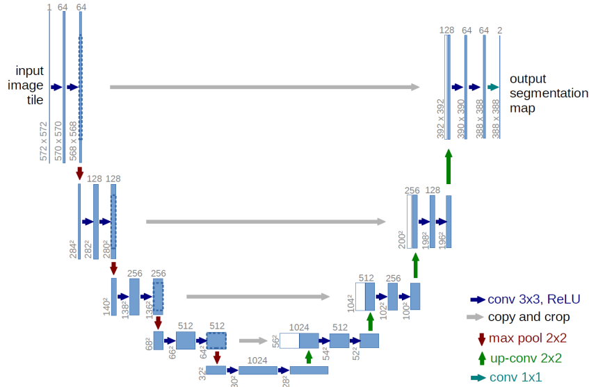
Figure 2.1: The U-Net architecture. The contracting path (left) progressively halves spatial resolution while doubling feature channels; the expanding path (right) restores resolution via transposed convolutions. Skip connections (horizontal arrows) carry fine-grained spatial features from encoder to decoder stages.
