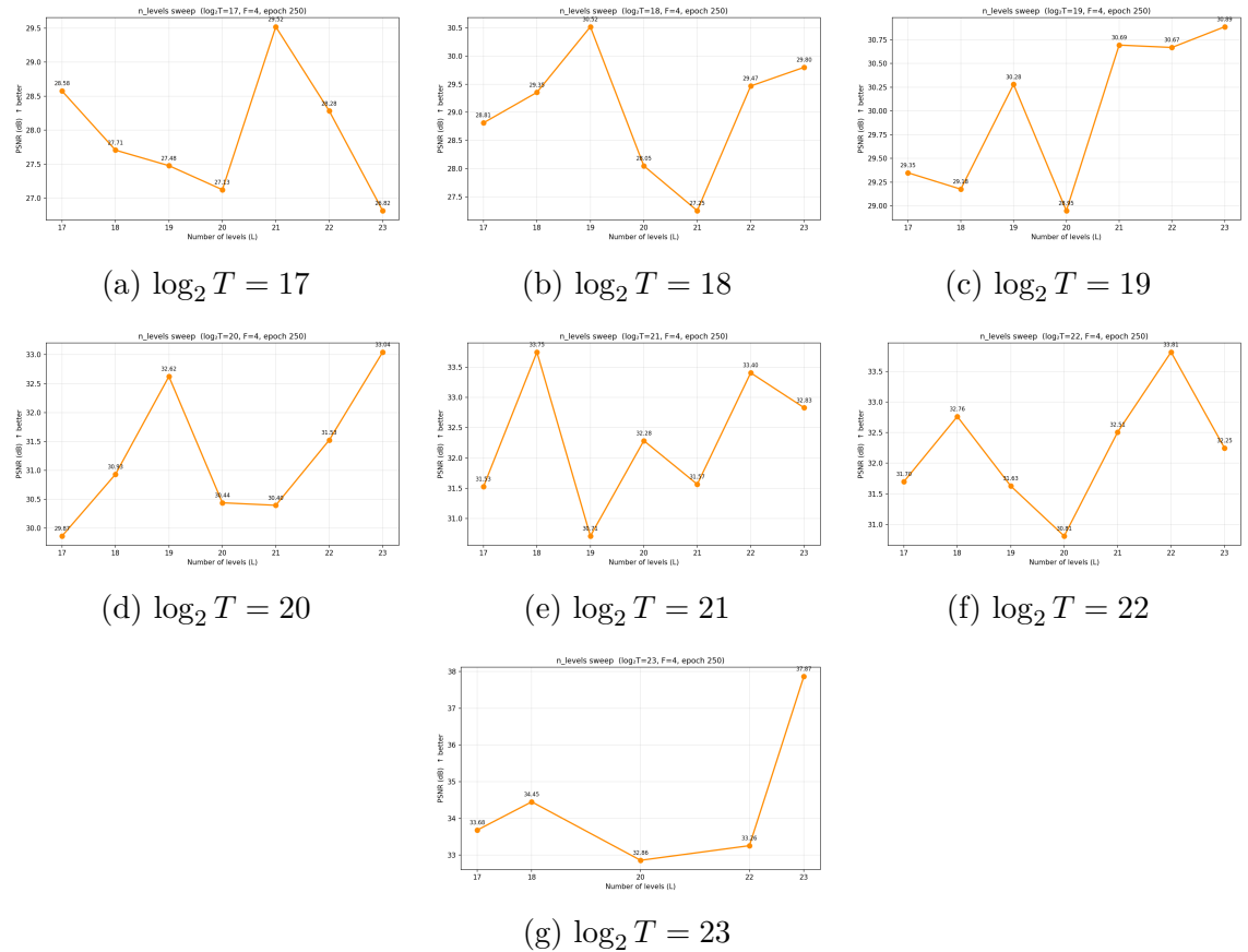
Figure 3.2: PSNR at epoch 250 as a function of number of levels L , with F = 4 fixed, shown separately for each \log_2 hashmap size. Each panel sweeps L \in \{17, \dots, 23\} with all other parameters held constant.
