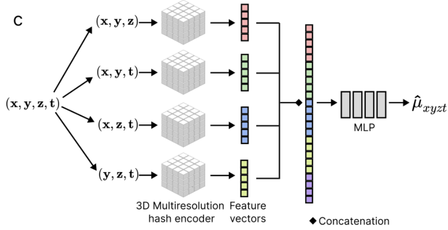
Figure 2.4: The NeCT QuadCubes architecture. Four independent 3D multiresolution hash encoders cover all four 3-element subsets of the space-time coordinates \{x, y, z, t\} . Their concatenated feature vectors are decoded by a shared MLP to produce the attenuation coefficient \hat{\mu}(\mathbf{r}, t) .
