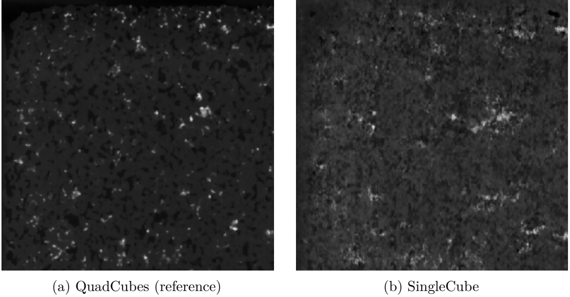
Figure 4.1: Reconstruction comparison between QuadCubes and SingleCube. The SingleCube output exhibits severe noise from the extreme hash collision load in the 4D encoder, while the QuadCubes decomposition into 3D subproblems produces a clean reconstruction.
