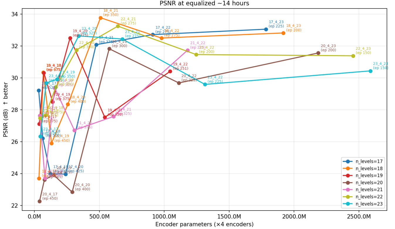
Figure 3.3: PSNR at an equalized training time of approximately 14 hours for all (L, \log_2 T) configurations with F = 4 . Each curve groups configurations with the same number of levels L ; x-axis shows total encoder parameter count across all four QuadCubes encoders.
