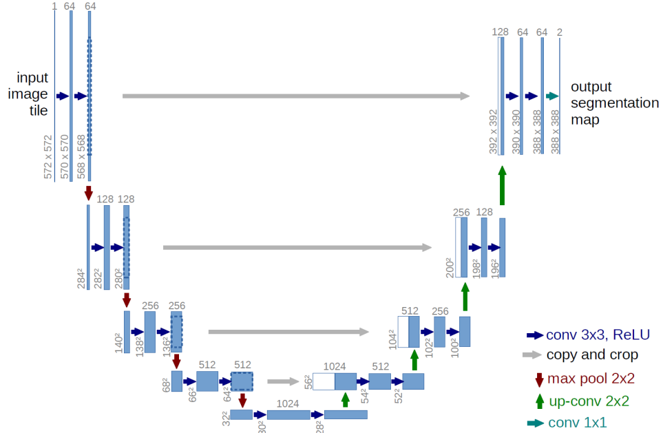
Figure 2.1: The U-Net architecture. The contracting path (left) progressively halves spatial resolution while doubling feature channels; the expanding path (right) restores resolution via transposed convolutions. Skip connections (horizontal arrows) carry fine-grained spatial features from encoder to decoder stages.
