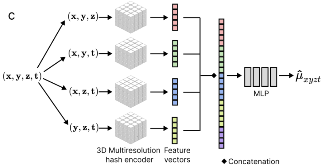
Figure 2.6: The NeCT QuadCubes architecture. Four independent 3D multiresolution hash encoders concatenating the feature vectors are decoded by a shared MLP.
