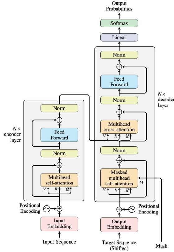
Figure 2.2: The Transformer architecture with encoder and decoder stacks. Each layer applies multi-head self-attention followed by a position-wise feed-forward network, with residual connections and layer normalisation at each sub-layer.
