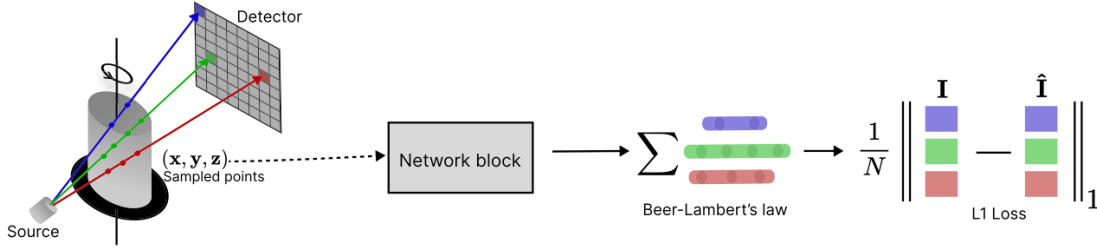
Figure 2.4: The NeCT training pipeline. Rays are sampled from recorded projections, marched through the hash-encoded network to predict attenuation values, integrated via the discretised Beer–Lambert law to produce predicted detector intensities, and compared to the measured intensities by the L1 loss. Gradients are backpropagated to update the network weights.
