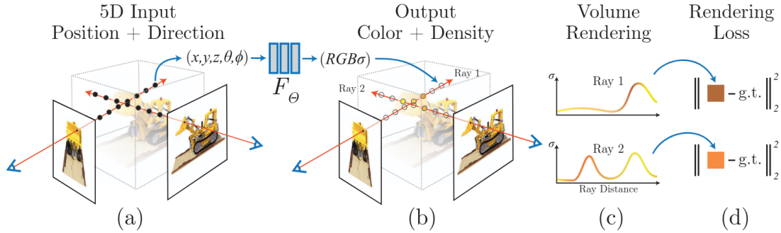
Figure 2.3: The NeRF pipeline. A continuous 5D function mapping spatial position and viewing direction to colour and density is represented by an MLP. Rays are marched through the volume, and the rendered pixel colour is compared to the observed image to supervise training via backpropagation.
