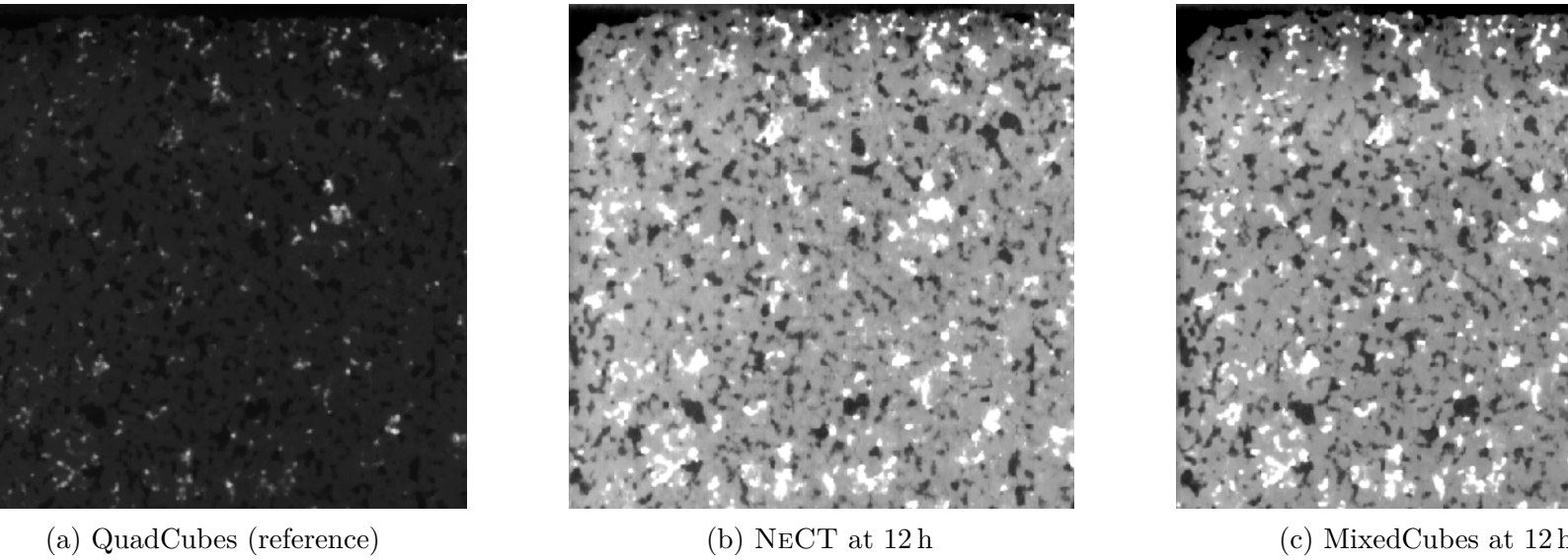
Figure 4.3: High-contrast reconstruction slices comparing the QuadCubes reference, uniform NECT configuration, and the non-uniform MixedCubes allocation at an equalized 12-hour training budget. Differences are most visible at high-contrast material boundaries.
