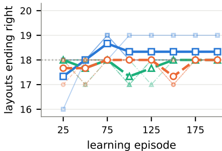
(a) frozen tree, 20 held-out layouts
