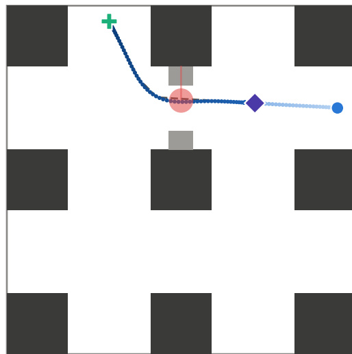
(b) gate: wait until the pedestrian has passed
