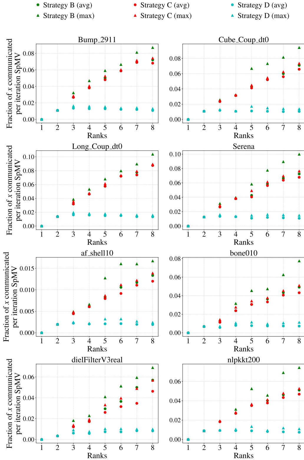
Figure 5.19: Fraction of the global x^{67} vector communicated per iteration of SpMV on 1–8 nodes (one MPI rank per node) using single-socket AMD EPYC 7302P processors.
