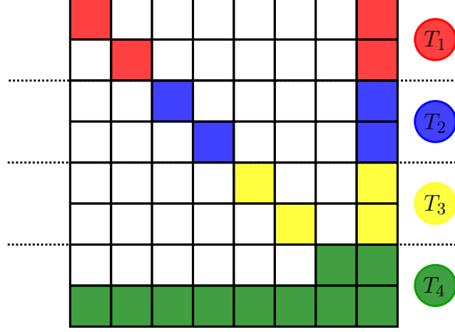
Figure 3.6: Row distribution among threads under static scheduling.
