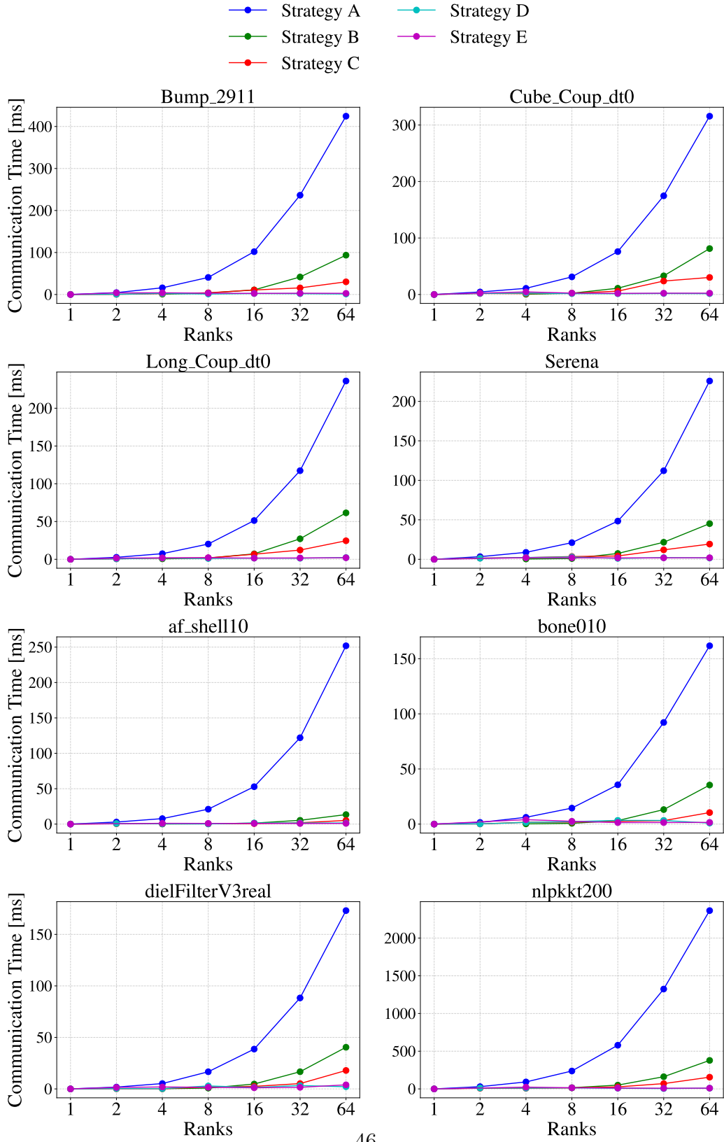
Figure 5.4: Communication time per iteraton of SpMV on a single node equipped with dual-socket AMD EPYC 7601 processors.
