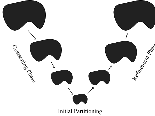
Figure 3.7: Illustration of multilevel graph partitioning (adapted from [6]).
