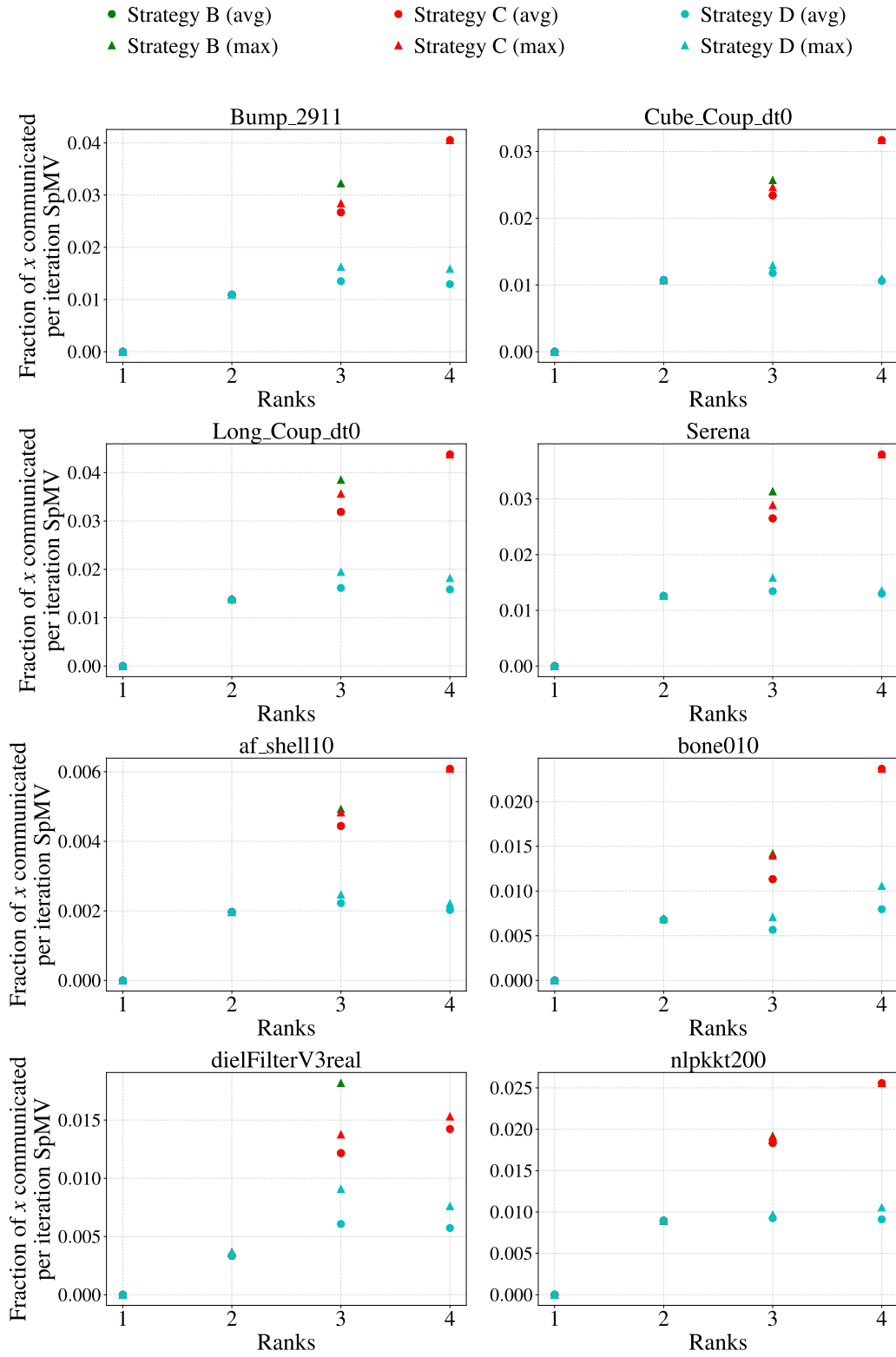
Figure 5.11: Fraction of the global x 56 vector communicated per iteration of SpMV on 1–4 nodes (one MPI rank per node) using dual-socket AMD EPYC 7601 processors.
