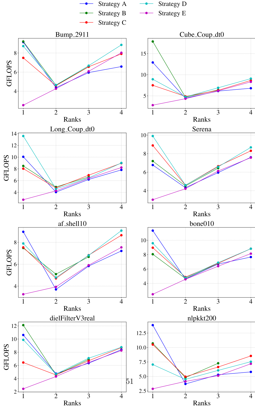
Figure 5.7: Sustained GFLOPS performance of SpMV over 100 iterations on 1–4 nodes (one MPI rank per node) using dual-socket AMD EPYC 7601
