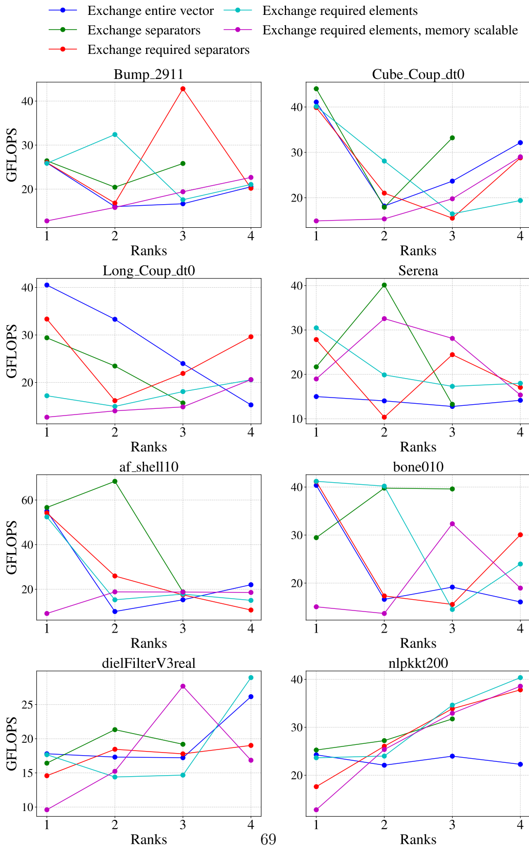
Figure 5.20: multi Node - AMD EPYC 7413
