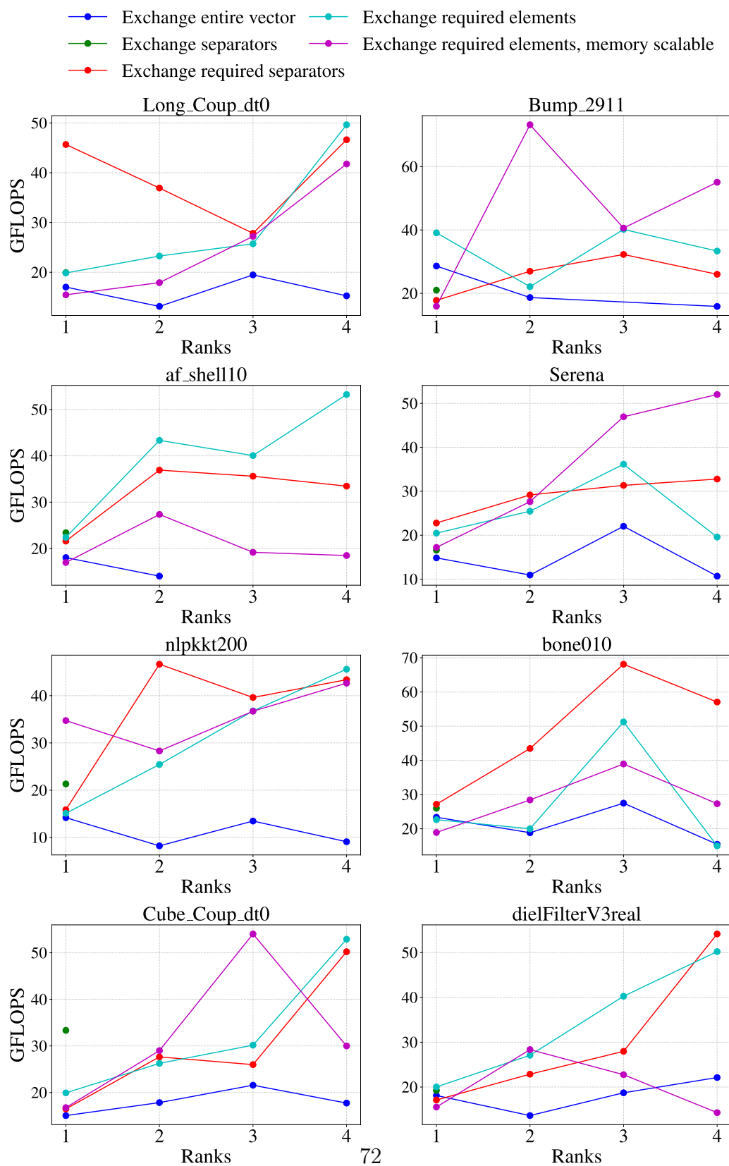
Figure 5.23: Multi Node - AMD EPYC 7413
