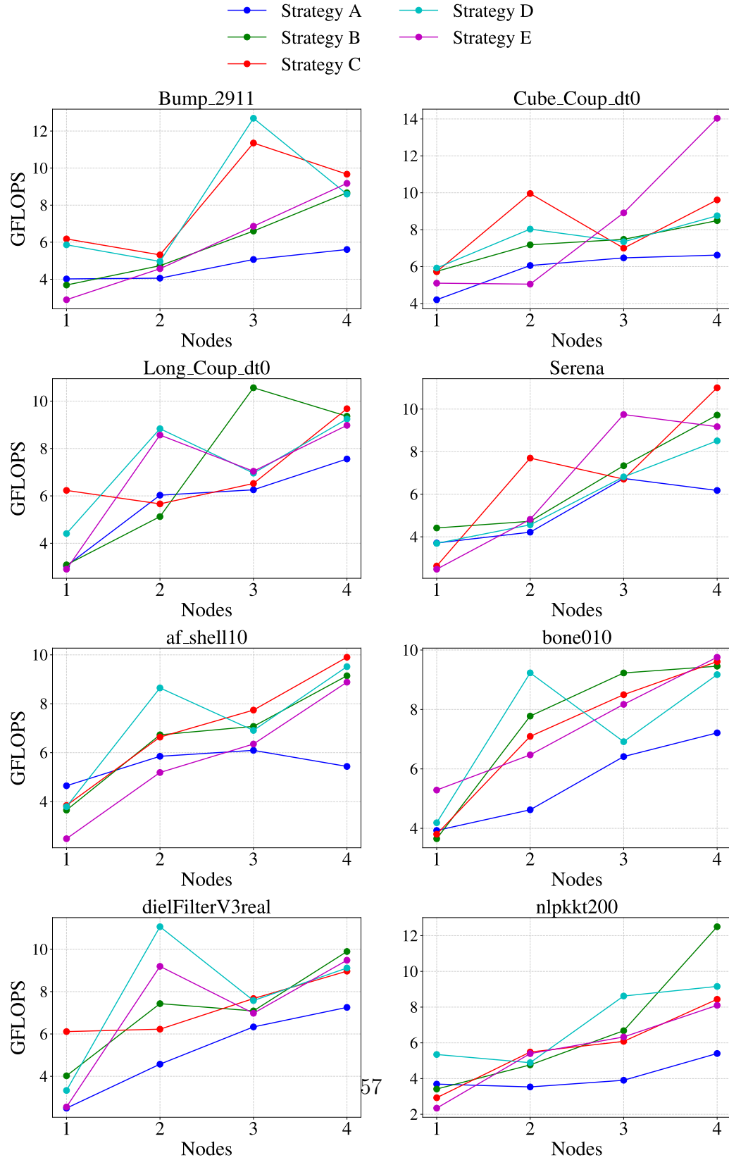
Figure 5.12: Sustained GFLOPS performance of SpMV over 100 iterations on 1-4 nodes (one MPI rank per socket) using dual-socket AMD EPYC 7601
