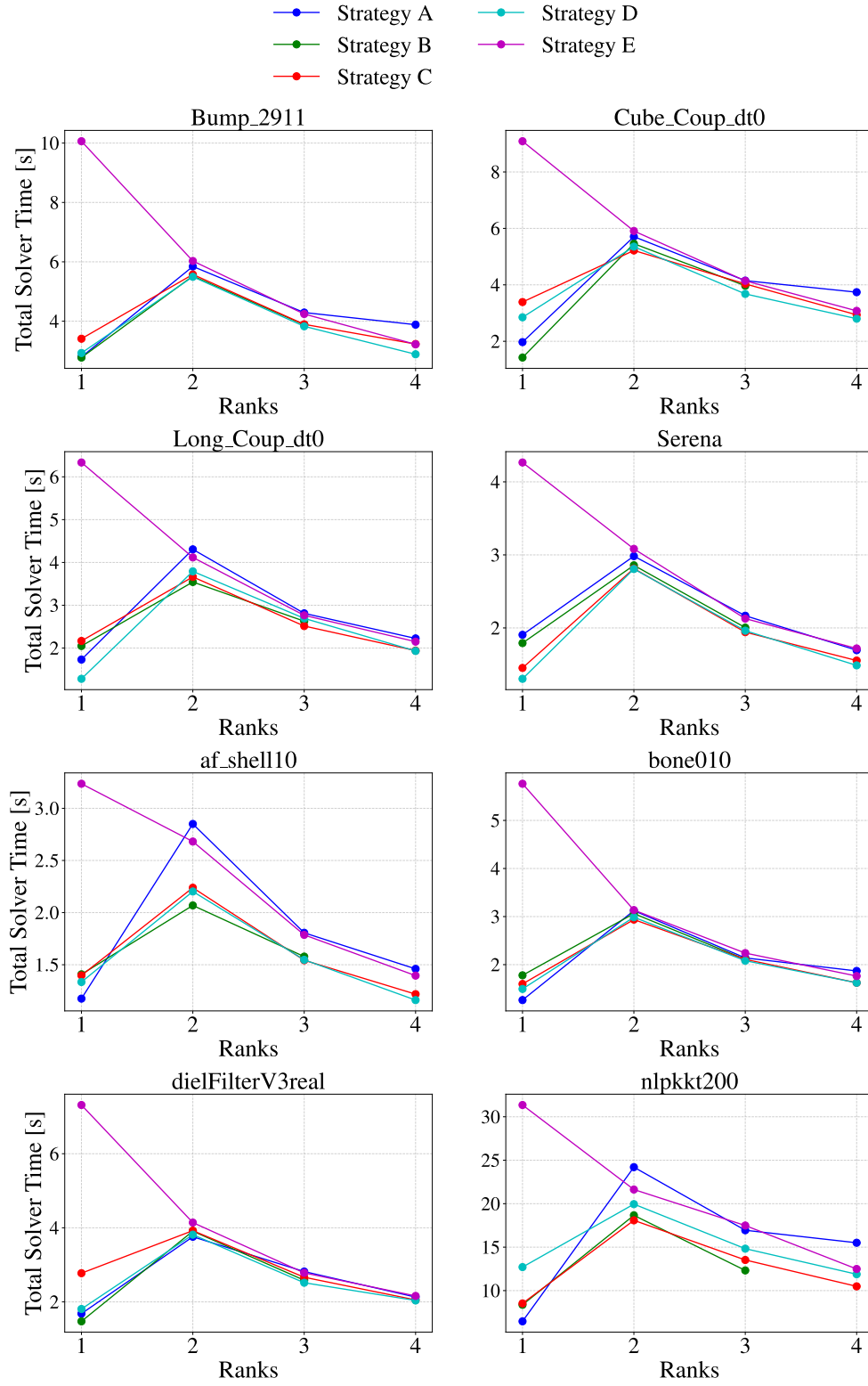
Figure 5.8: Total execution time for 100 iterations of SpMV on 1–4 nodes (one MPI rank per node) using dual-socket AMD EPYC 7601 processors.
