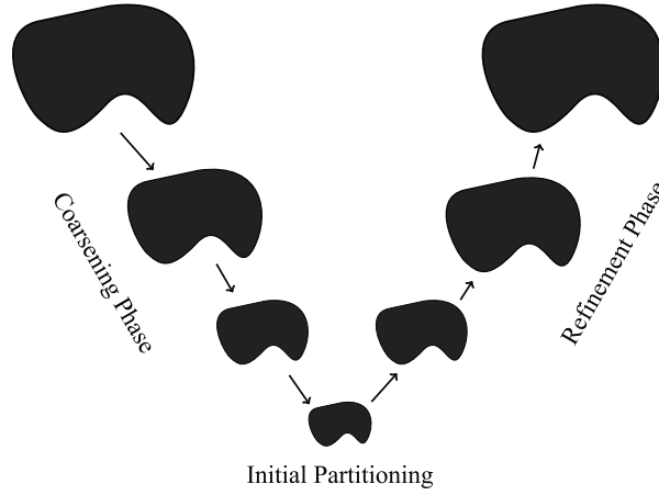
Figure 3.7: Illustration of multilevel graph partitioning (adapted from [9]).
