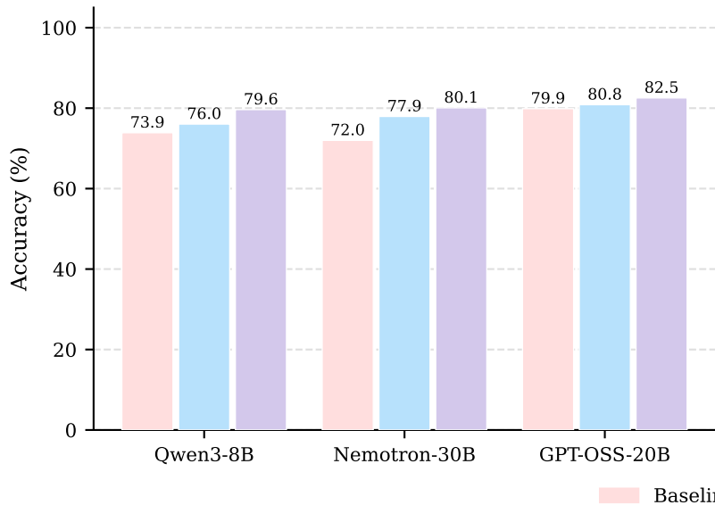
(a) Accuracy on Biased Prompts
