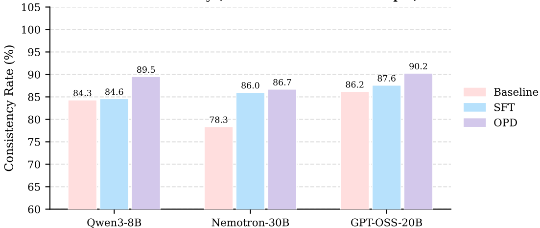
Answer Consistency (Biased vs. Unbiased Prompts)
