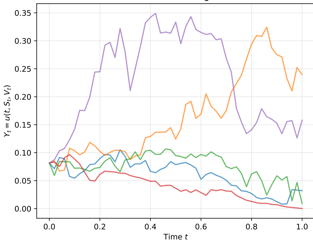
NN Predictions Along Paths
