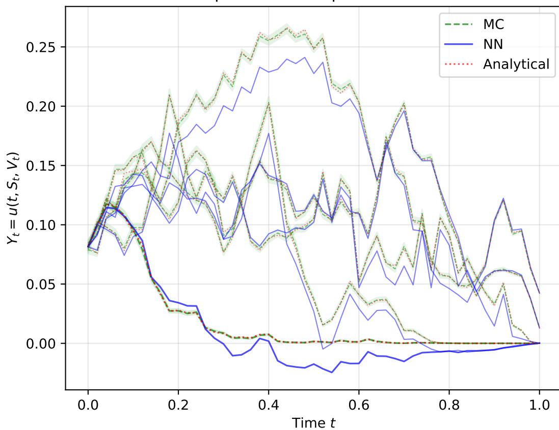
NN Predictions Along Paths
