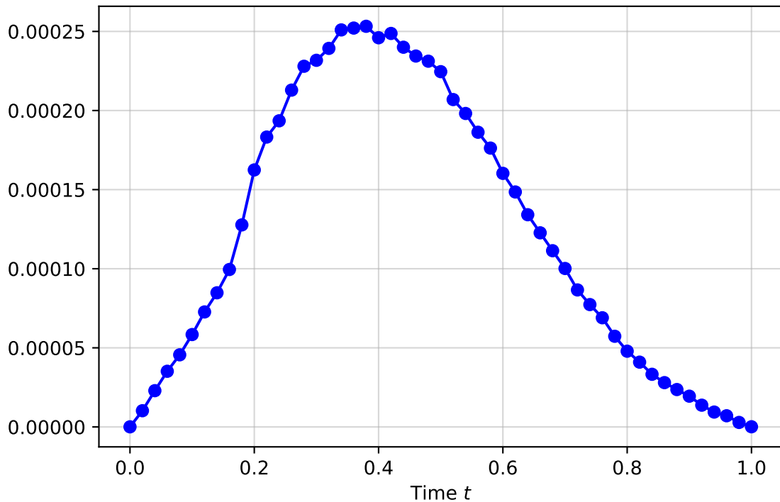
MSE over time (Naisnet - Sine, \rho=-0.5 , M=100 )
