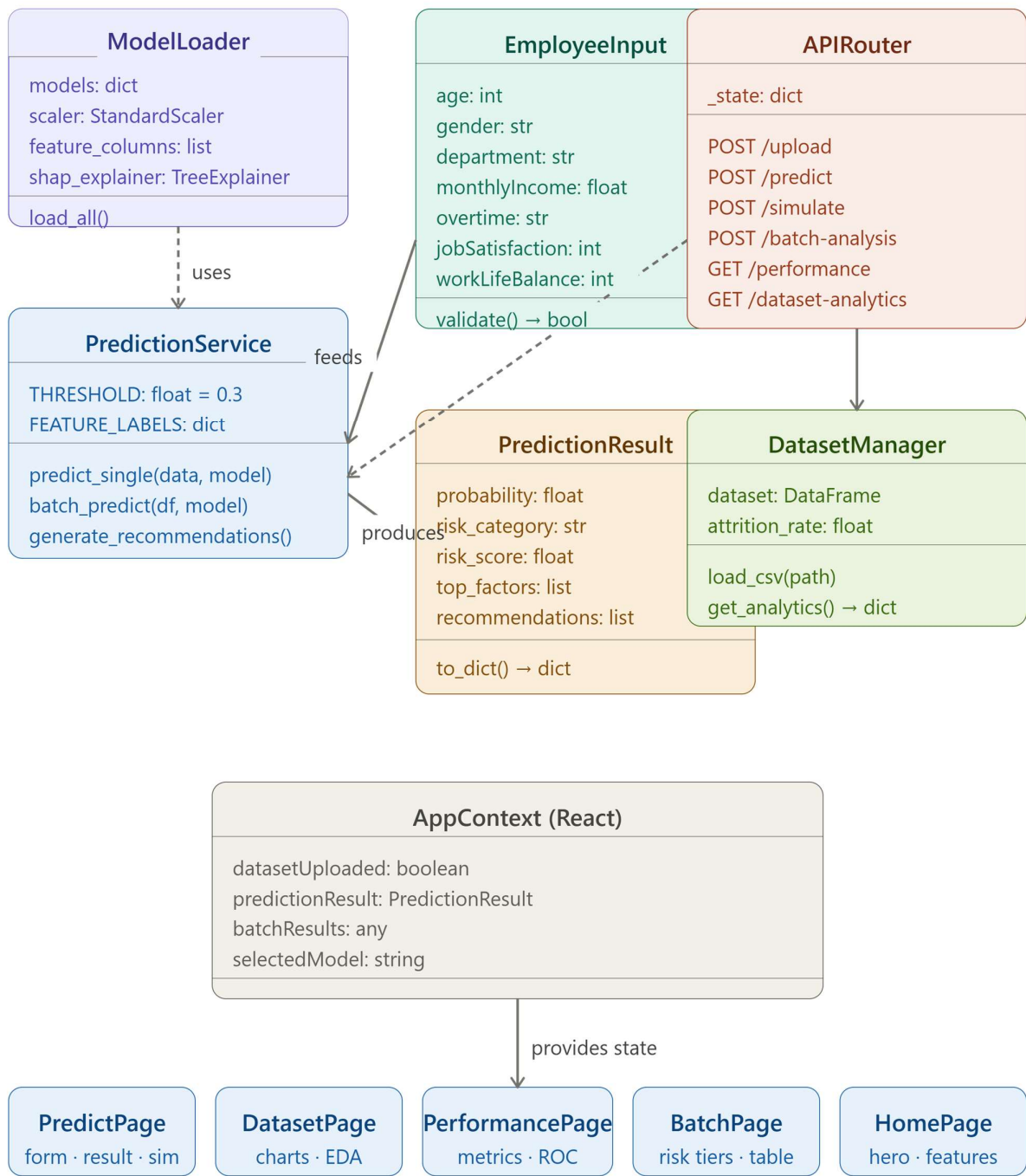
UML class diagram
