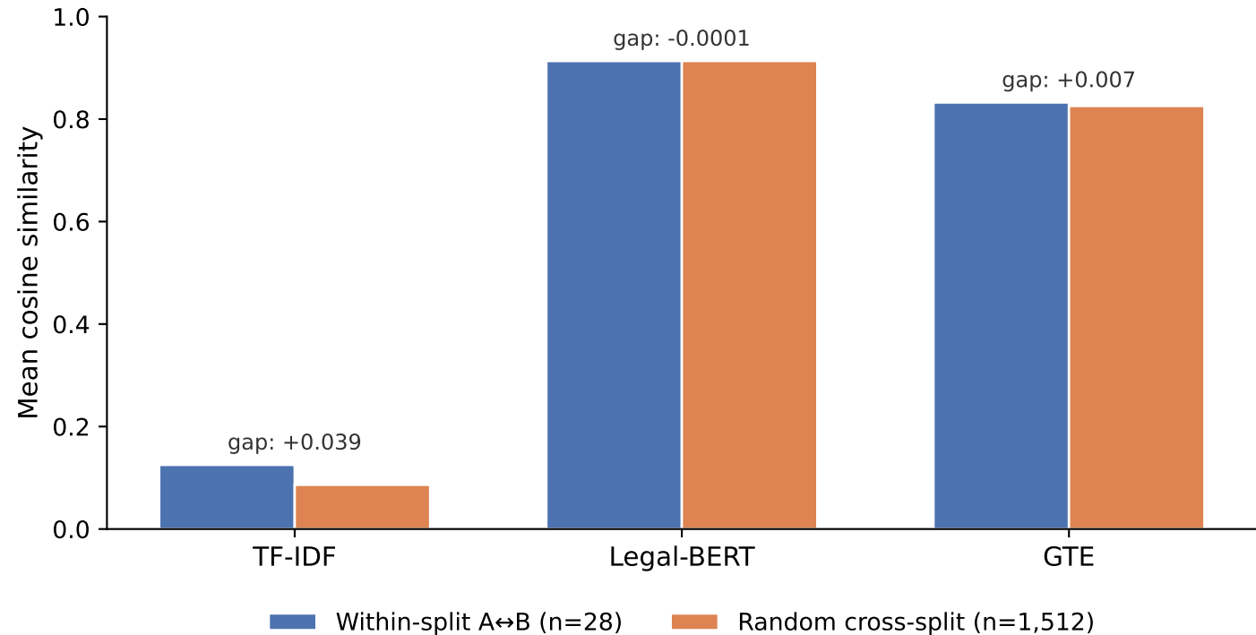
Within-split A↔B vs. random baseline similarity, by model
