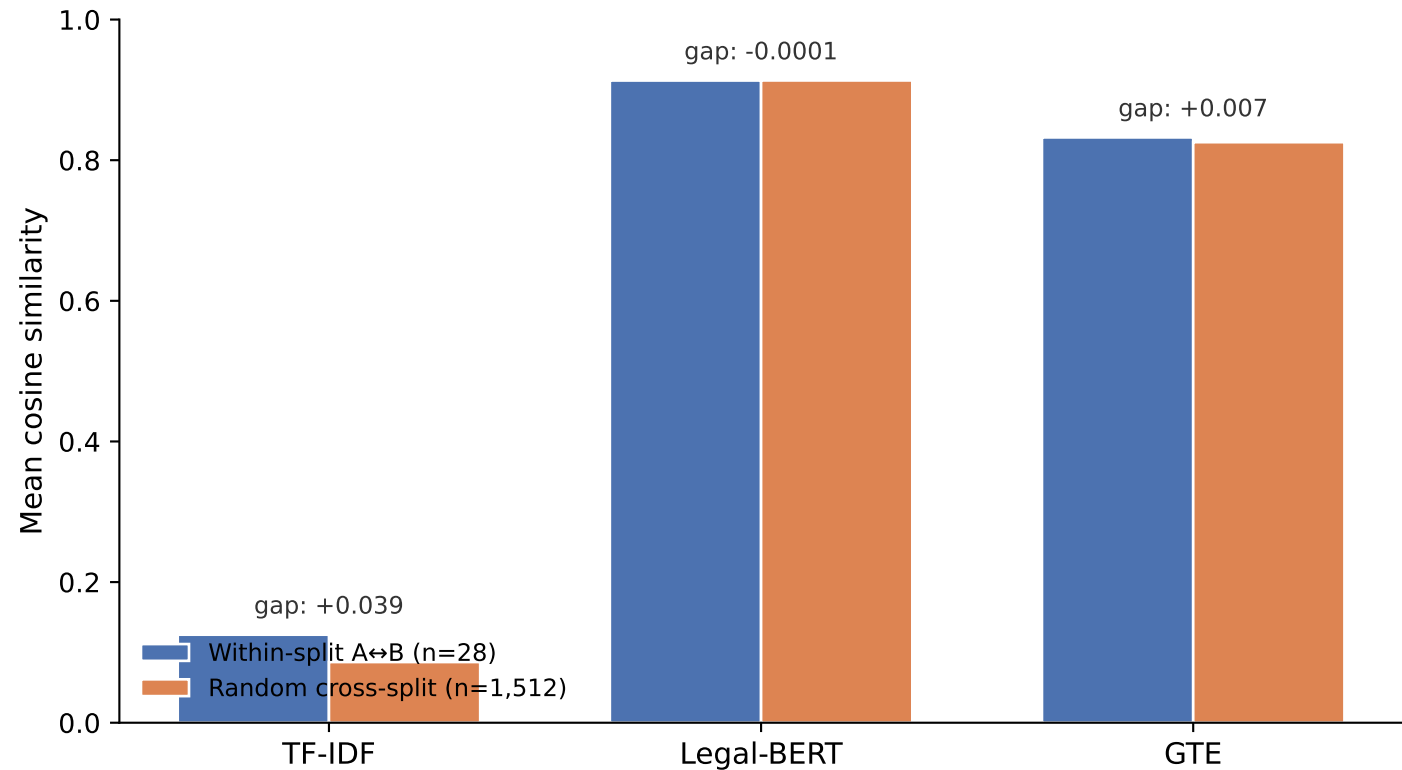
Within-split A↔B vs. random baseline similarity, by model
