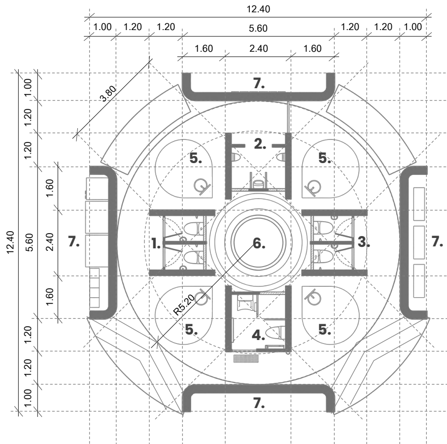
Floor plan
