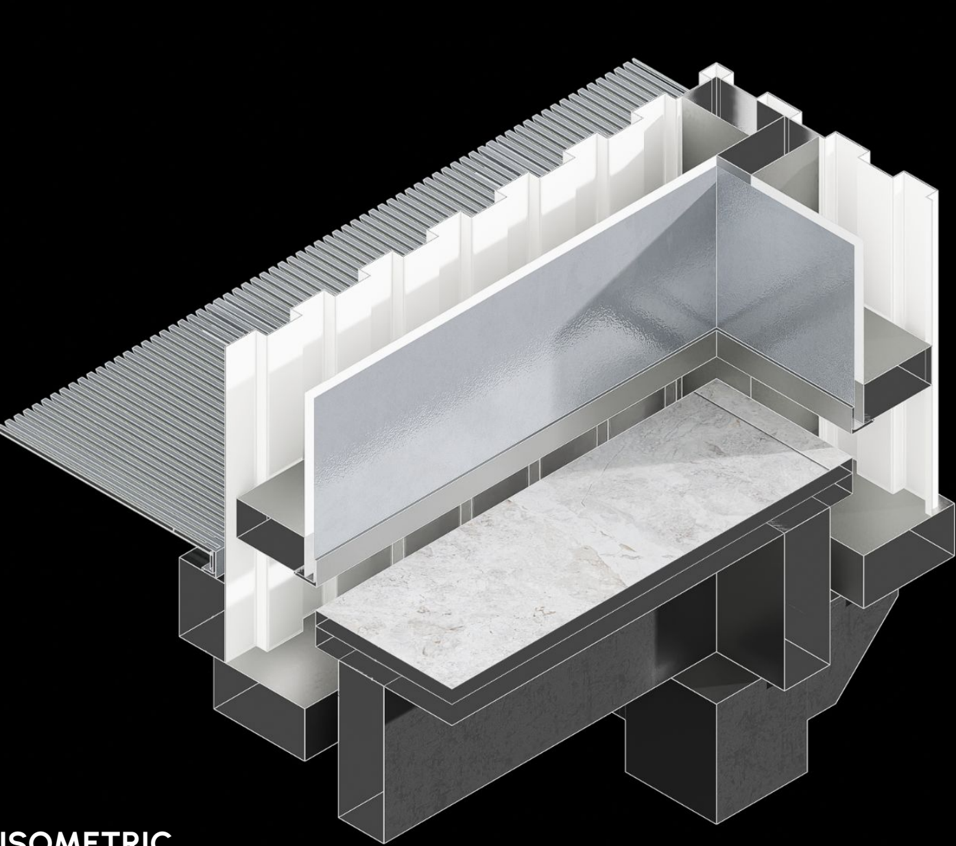
ISOMETRIC WALL BOTTOM
