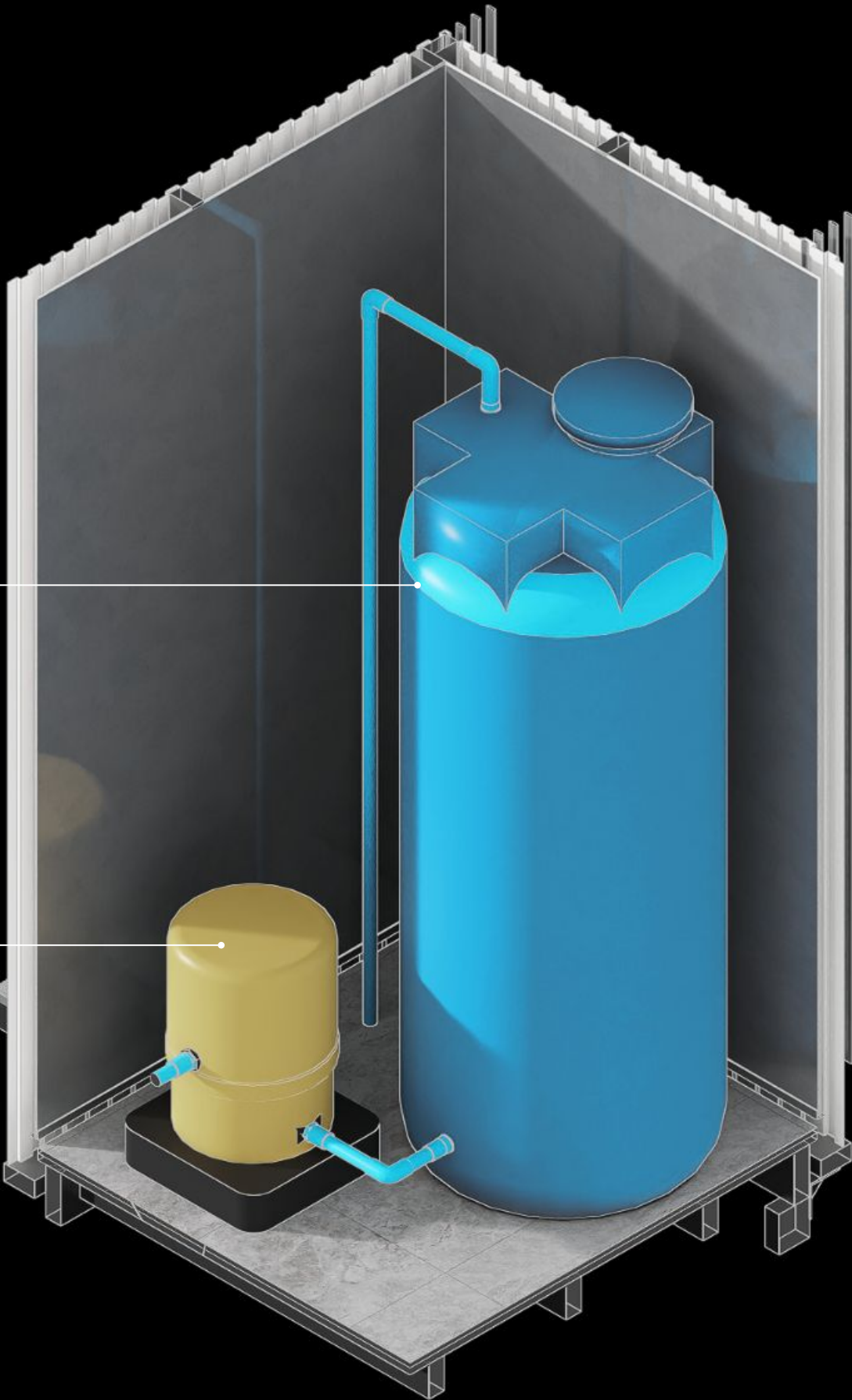
ISOMETRIC PUMP MODULE
