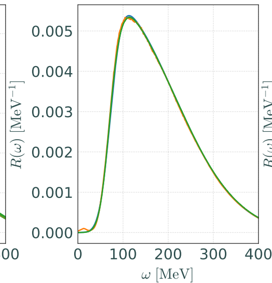
Noise level: 0.0001
