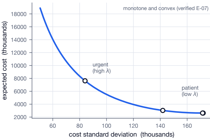
(c) Efficient frontier of execution
