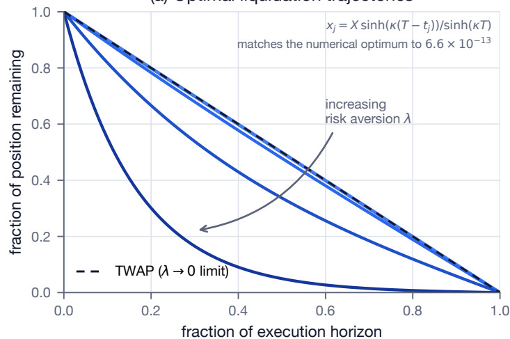
(a) Optimal liquidation trajectories
