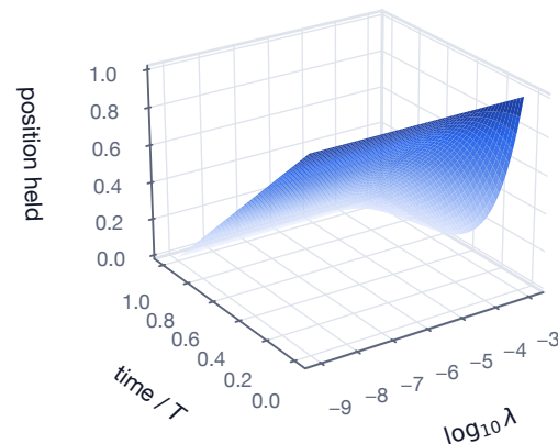
(b) Trajectory surface
