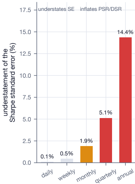
(b) Using EXCESS kurtosis by mistake
