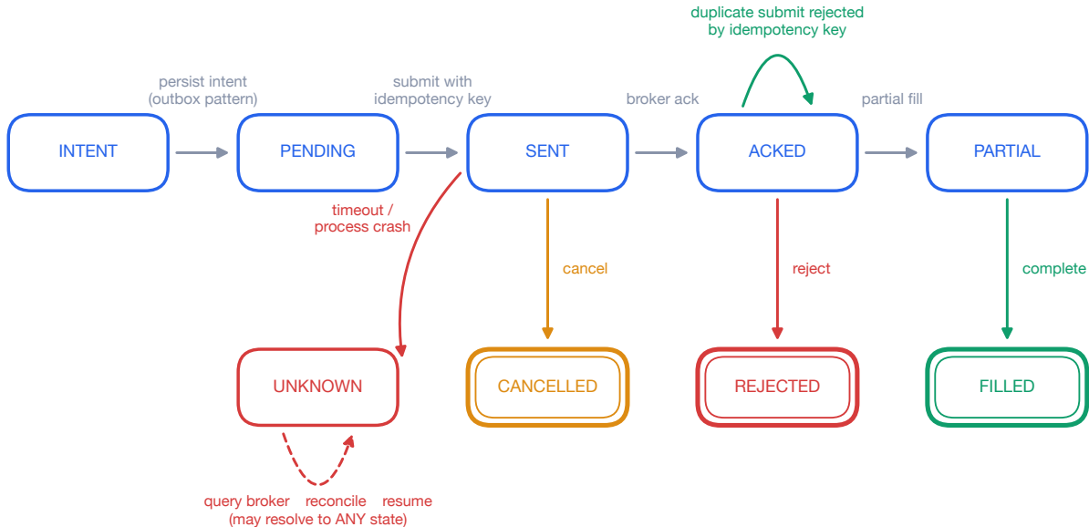
Figure 10 — Order lifecycle: every transition persisted, every submission idempotent
