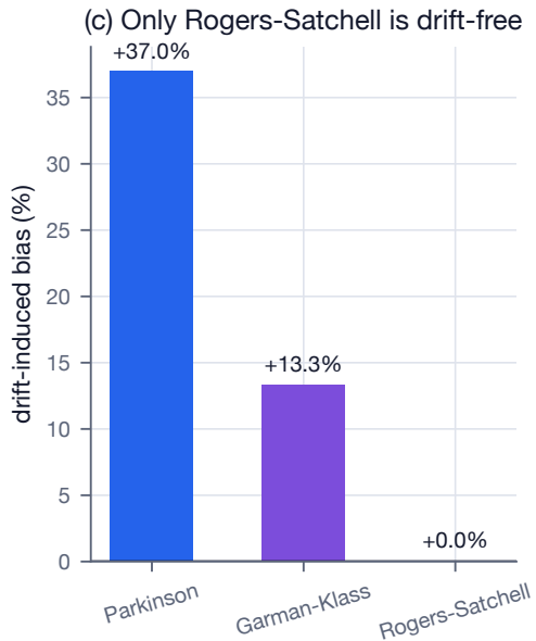
Figure 16 — Range-based volatility estimators: correct in theory, biased on real bars
