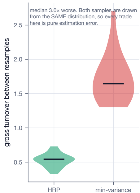
Rebalancing forced by noise alone
