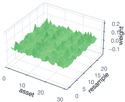
Hierarchical Risk Parity
