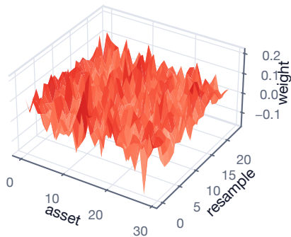
Minimum variance ( \Sigma^{-1} )
