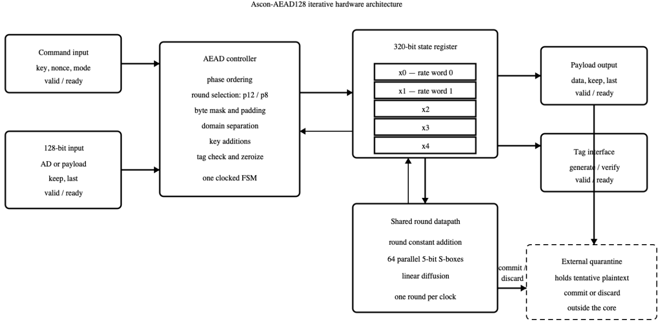
Byte lane 0 is bits 7:0. The same datapath serves initialization, associated data, payload, and finalization.
