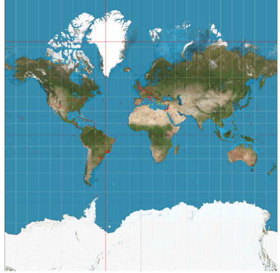
Figure 5. Greenland real size and Mercator country size distortion
