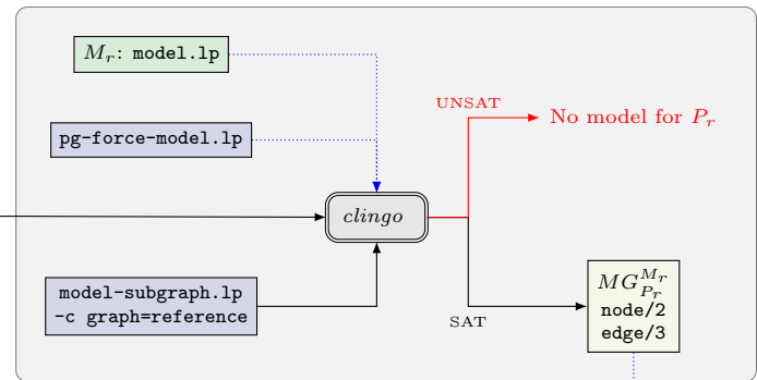
② Construct MG_{P_r}^{M_r} .
