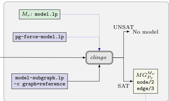
Construct MG_P^M
