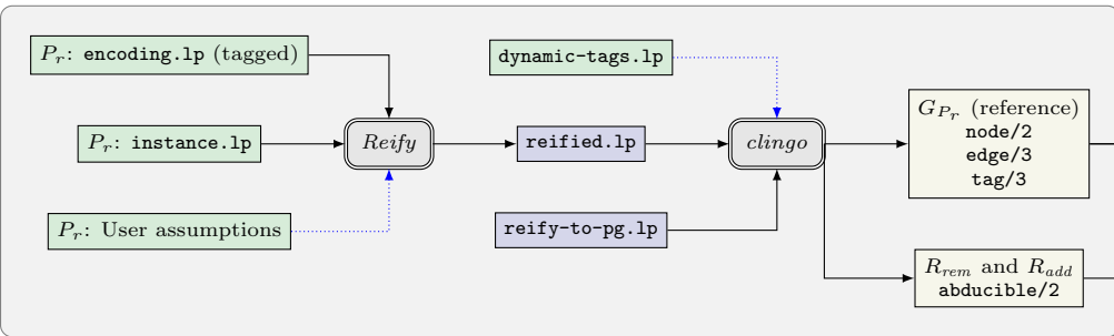
Construct G_P
