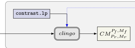
④ Construct CM_{P_r, M_r}^{P_f, M_f} .
