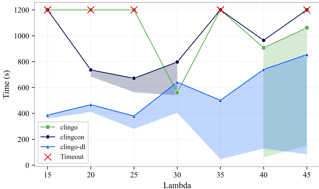
RANDOM - Timepoint limit = 100
