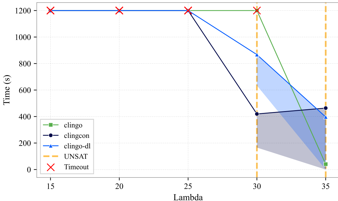
RANDOM - Timepoint limit = 30
