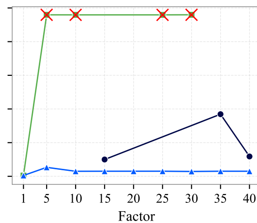
Agents = 3
