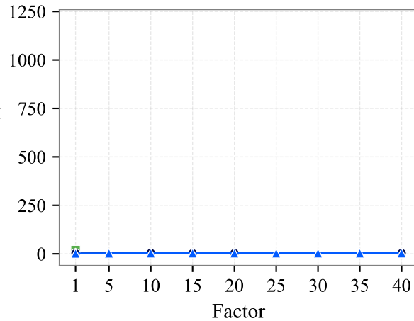
Agents = 1
