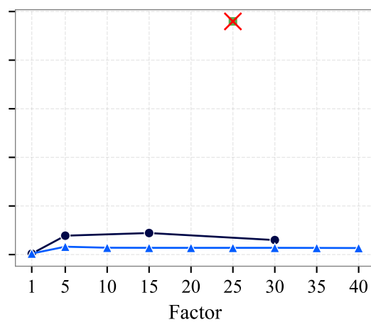
Agents = 2
