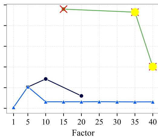
Agents = 4
