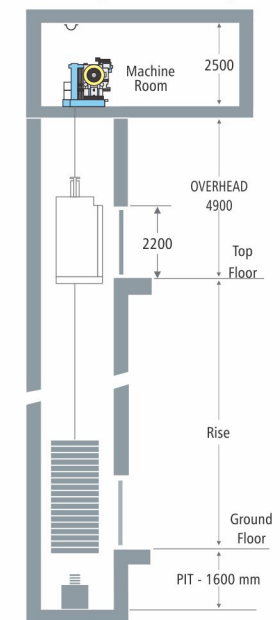
Hoistway Elevation Drawing
