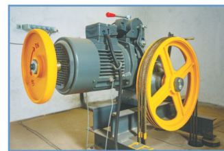
Heavy Duty Traction Machine
