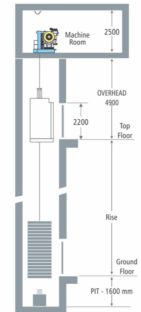
Hoistway Elevation Drawing
