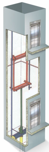
Direct Central Acting
