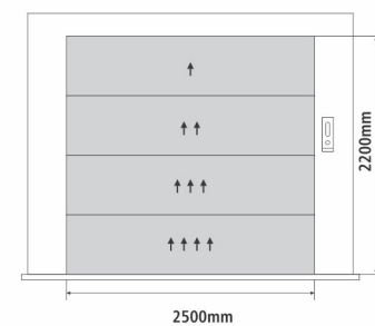
Vertical Opening Automatic Landing Door
