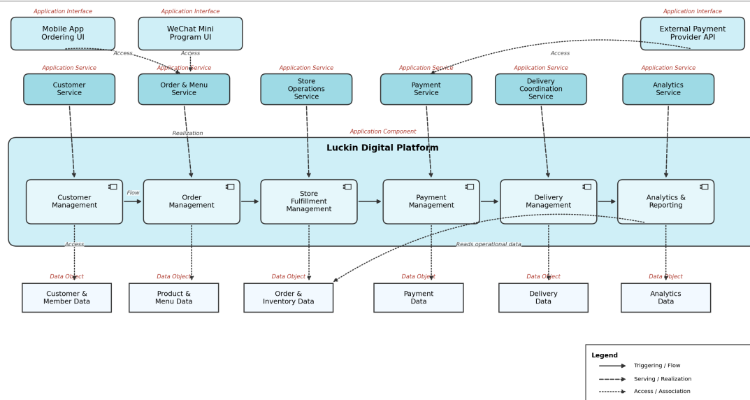
Figure 10: Application Layer Model from Seminar 6.
