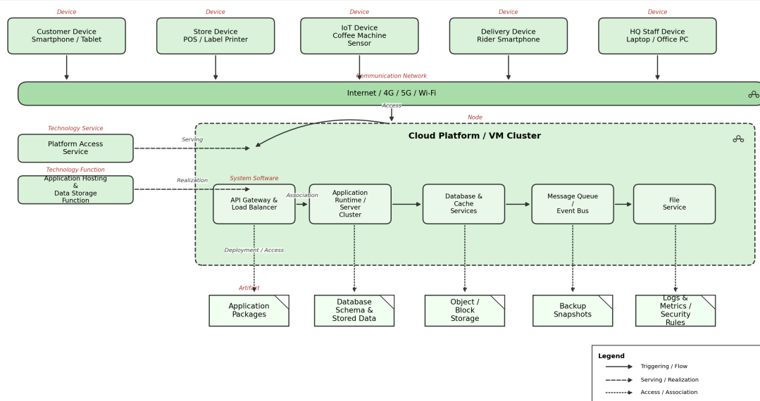
Figure 11: Technology Layer Model from Seminar 6.
