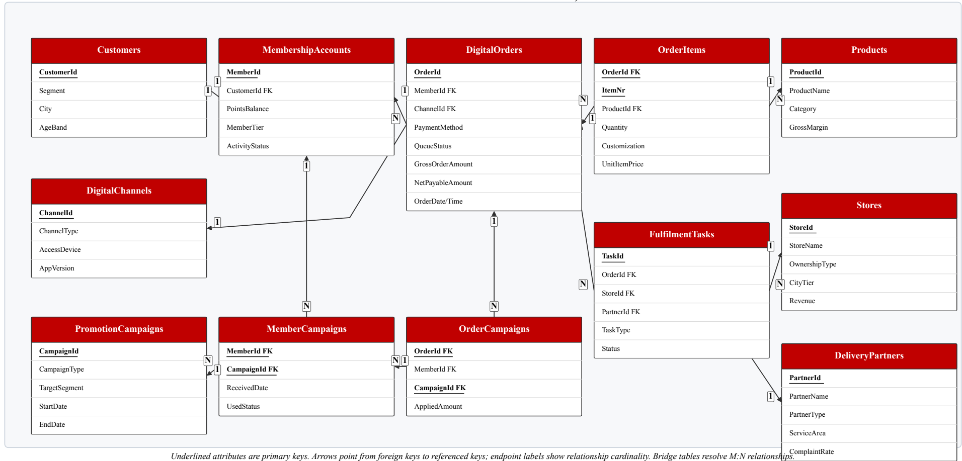
Figure 1: Relational data model diagram for customer, order, campaign, and fulfilment relations. Underlined attributes are primary-key attributes; FK marks foreign-key references; endpoint labels show cardinality, while bridge tables resolve M:N relationships.
