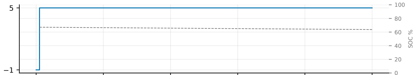
Proposed SPOTIS-MCDM
