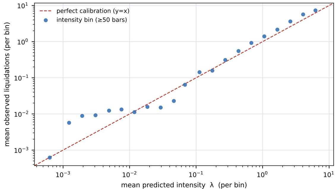
Aave v3 · branching n=0.66 (stationary ✓) · PIT KS D=0.0005
