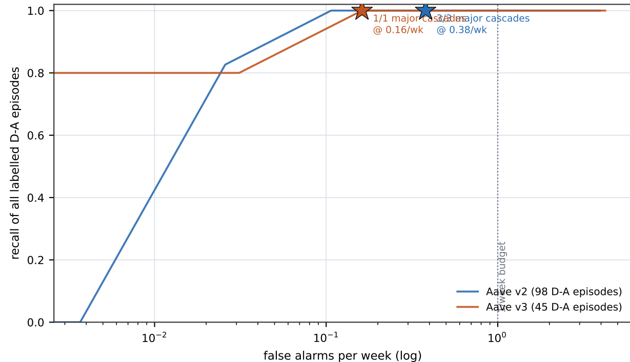
Threshold trade-off @ deployed debounce k (★ = operating point)
