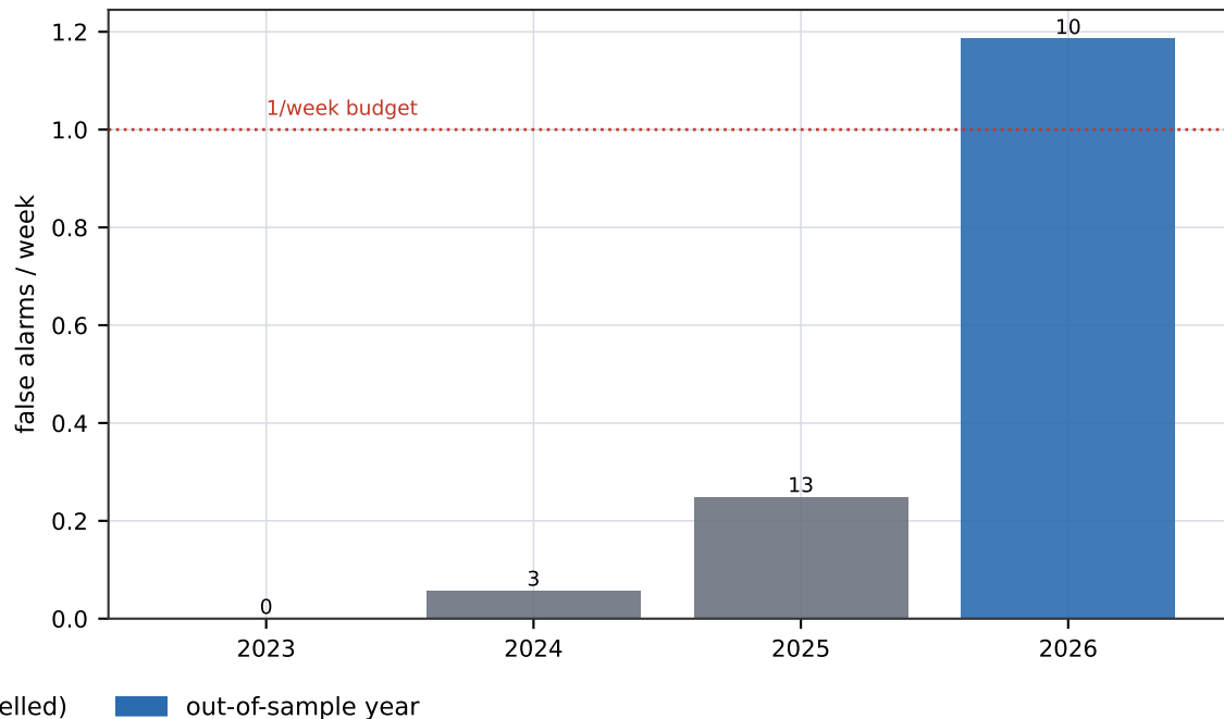
Aave v3 (k=10) — pooled OOS FAR = 0.18/week
