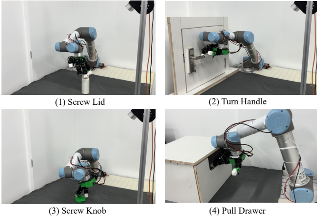
Fig. 7: Real-world deployments across 4 tasks.
