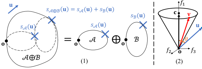
Fig. 2: Method illustration. (1) The support mapping s_A(\mathbf{u}) and its Prop. 3. (2) s_F(\mathbf{u}) for PCF contact model in 3D.
