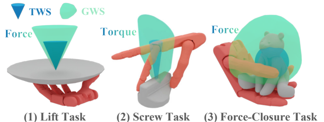
Fig. 1: Task-oriented dexterous hand poses synthesized for 3 tasks. Each TWS is specified by humans as a task prior: (1) the lift task requires upper forces, (2) the screw task requires counter-clockwise torques, and (3) the force-closure task requires wrenches in all directions. The GWS is computed based on the contacts between the hand and the object. Both TWS and GWS are visualized by their 3D force or torque components.
