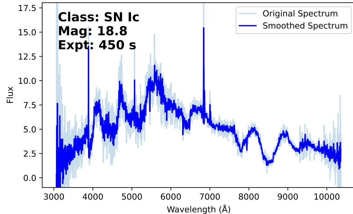
Spectrum from ZTF26aajqbmw
