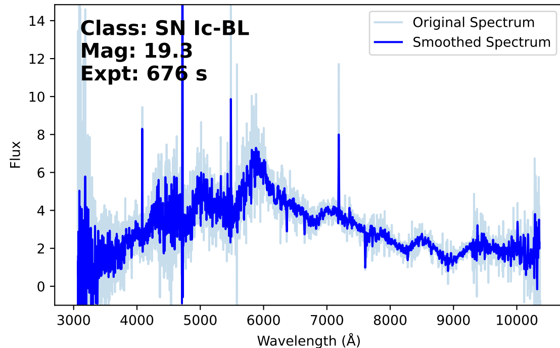
Spectrum from ZTF26aajrjtr
