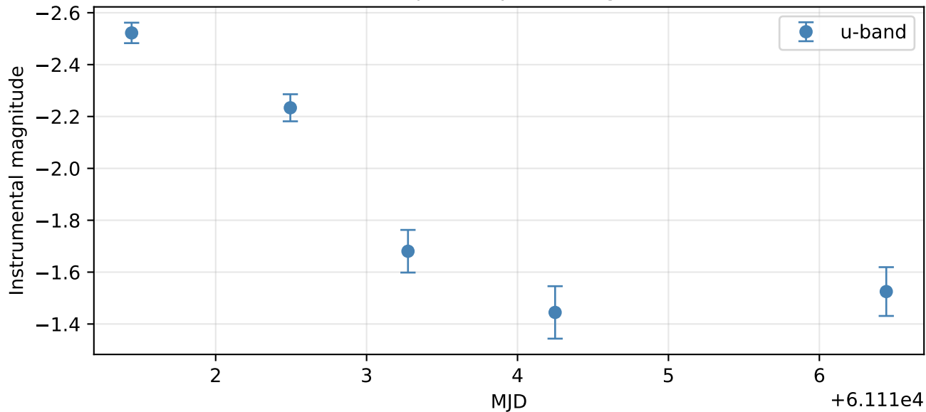
ZTF26aakjzdt - aperture light curve
