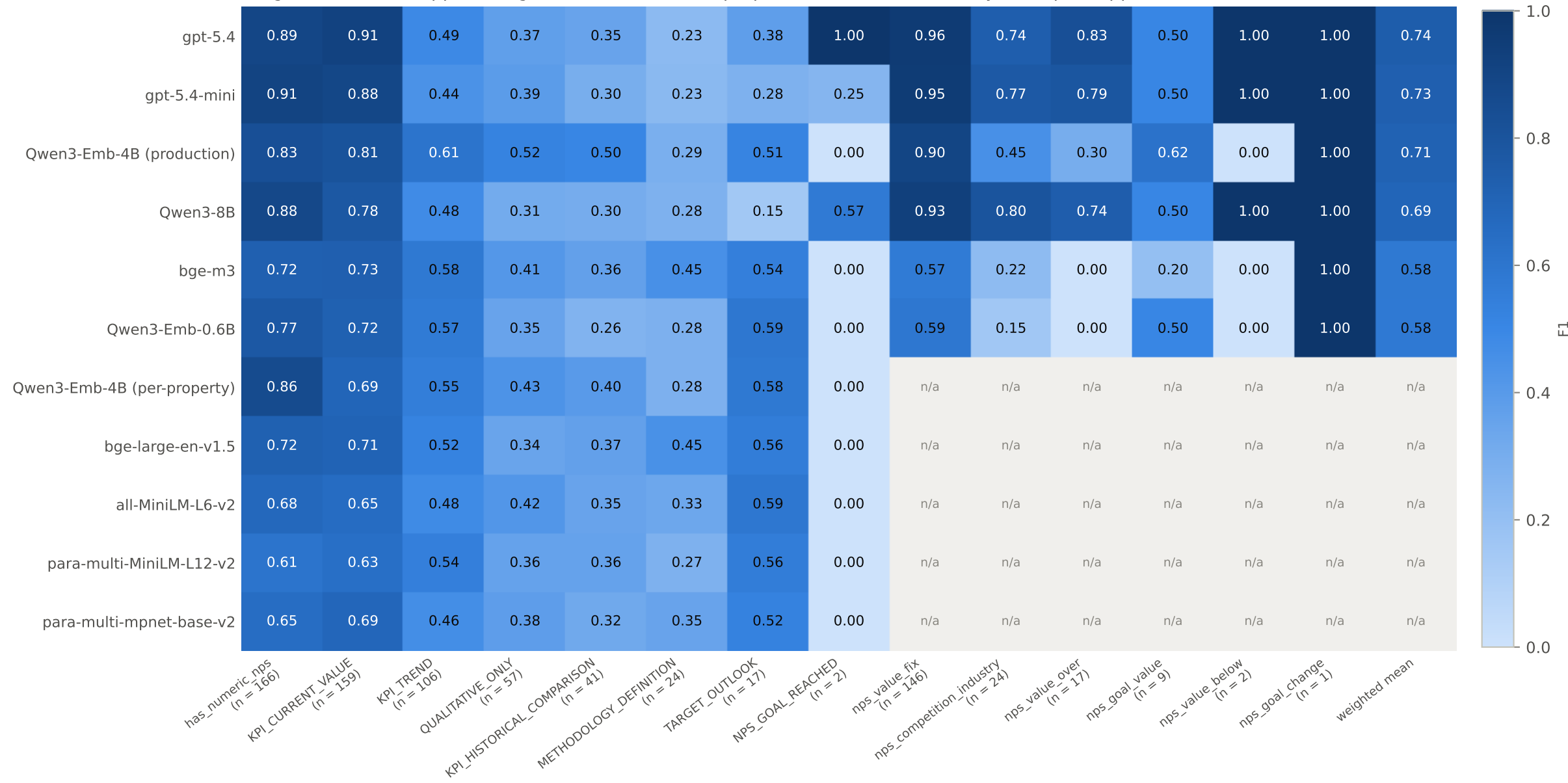
All 14 properties - F1 per property weighted mean = support-weighted over the shown properties; columns sorted by test-split support (n)
