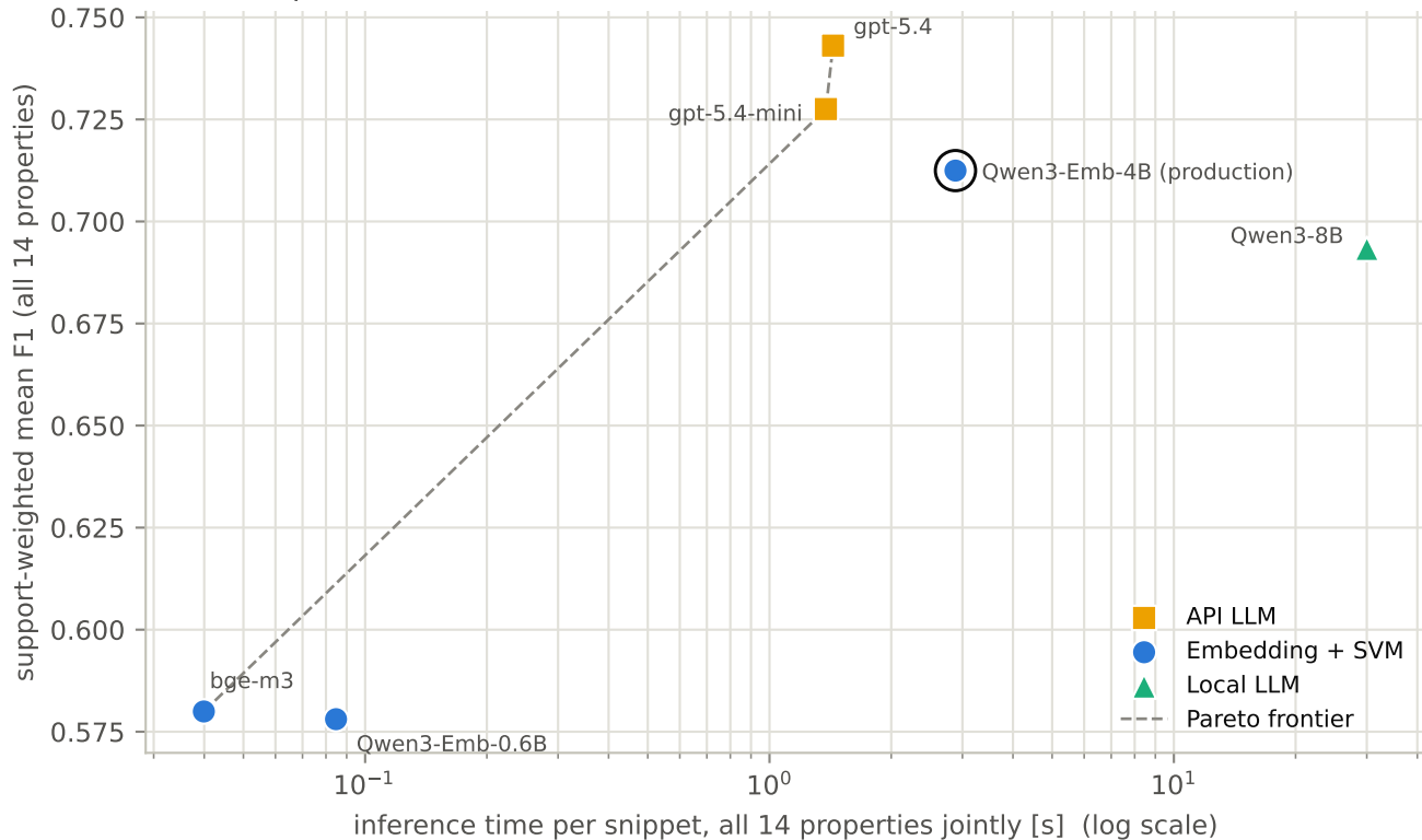
Quality vs. speed - all comparable models with full coverage circled = production model
