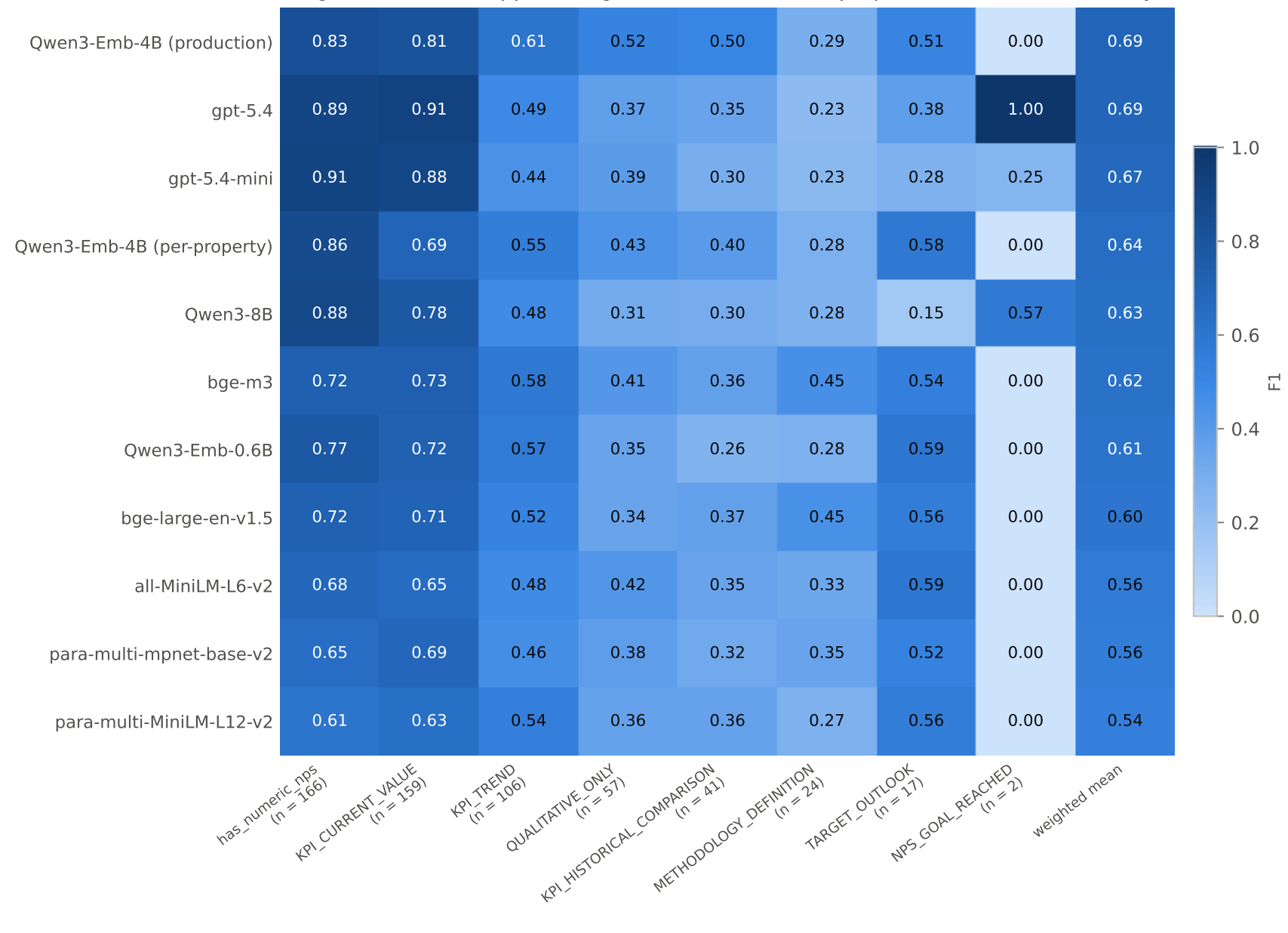
Boolean properties - positive-class F1 per label weighted mean = support-weighted over the shown properties; columns sorted by evaluation-split support (n)
