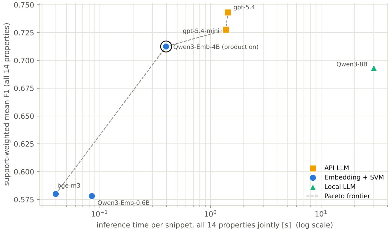
Quality vs. speed - all comparable models with full coverage circled = production model
