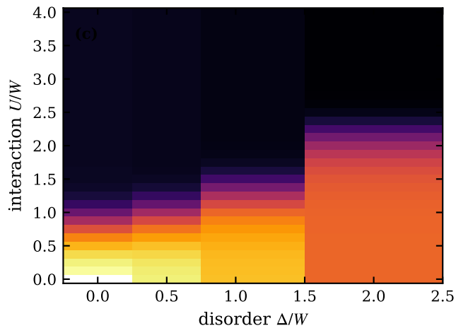
arith, n_c=0.49 , T/W=0.1 , \lambda=0
